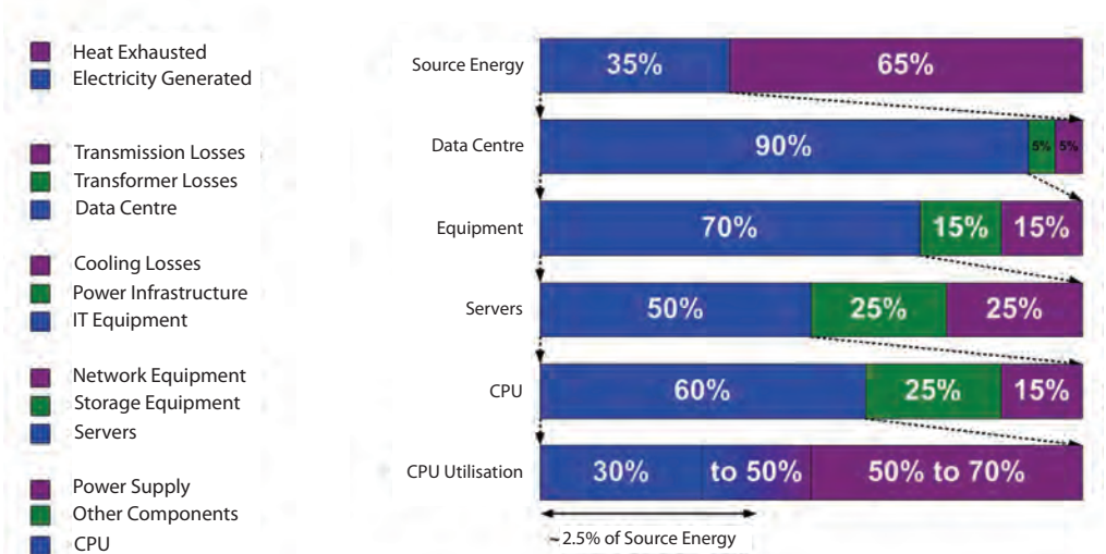
Figure 3: Diagram showing where energy is lost between source and processor in a 2012 style data centre (image courtesy of Liam Newcombe)
