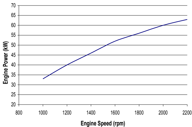
JCB Dieselmax 63kW Power Curve
